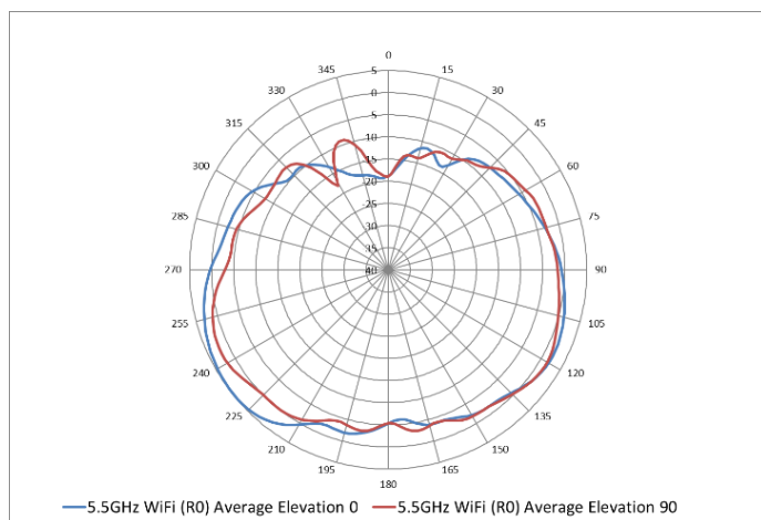
5.5GHz Wi-Fi antenna patterns (vertical)
